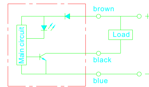
Wiring diagram (TC-11N)
