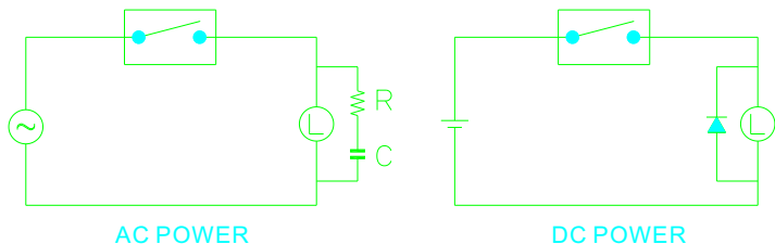
Additional external protection circuit
