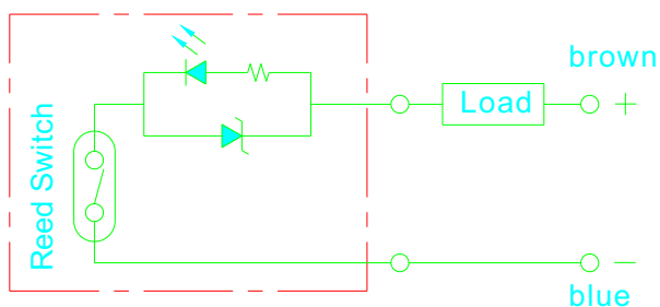
Wiring diagram (TC-22)
