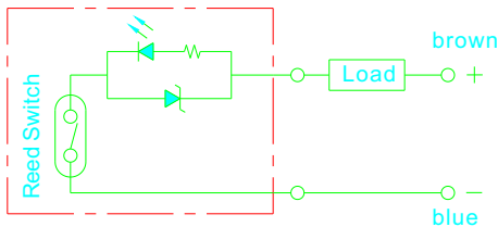
Wiring diagram
