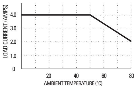
Max. Load Current vs. Temp.
